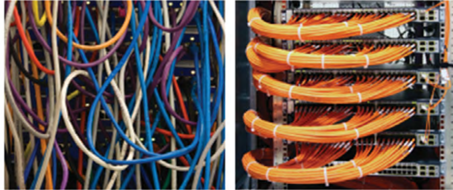
Figure 4: Structured Cabling Improves Air Circulation to Servers
